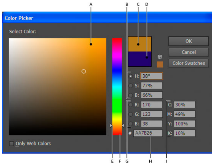
Color Picker
