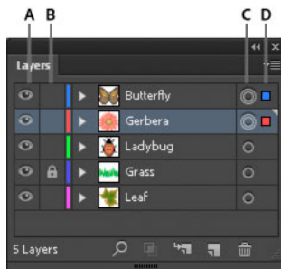
Layers panel
