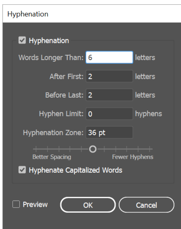
Hyphenation options
