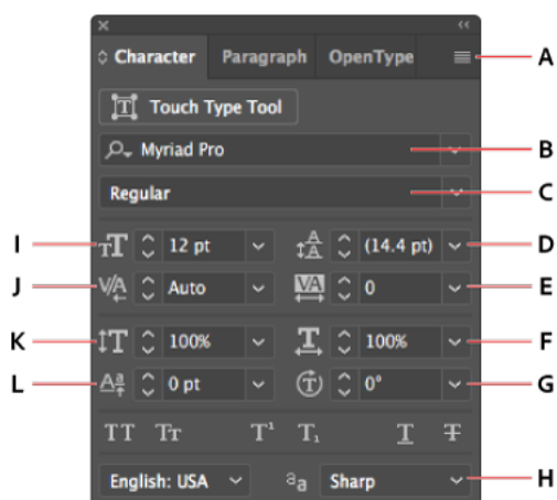
Character panel
