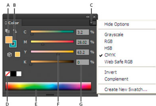
Color panel
