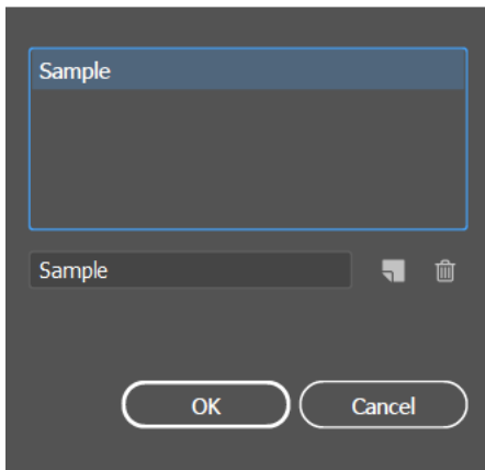
Manage Toolbar
