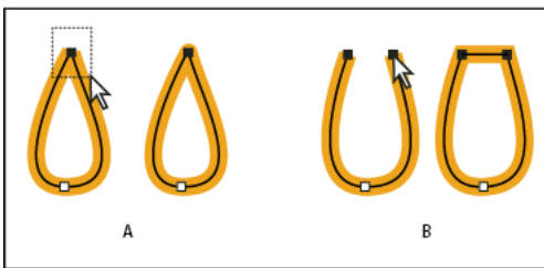
Joining endpoints
